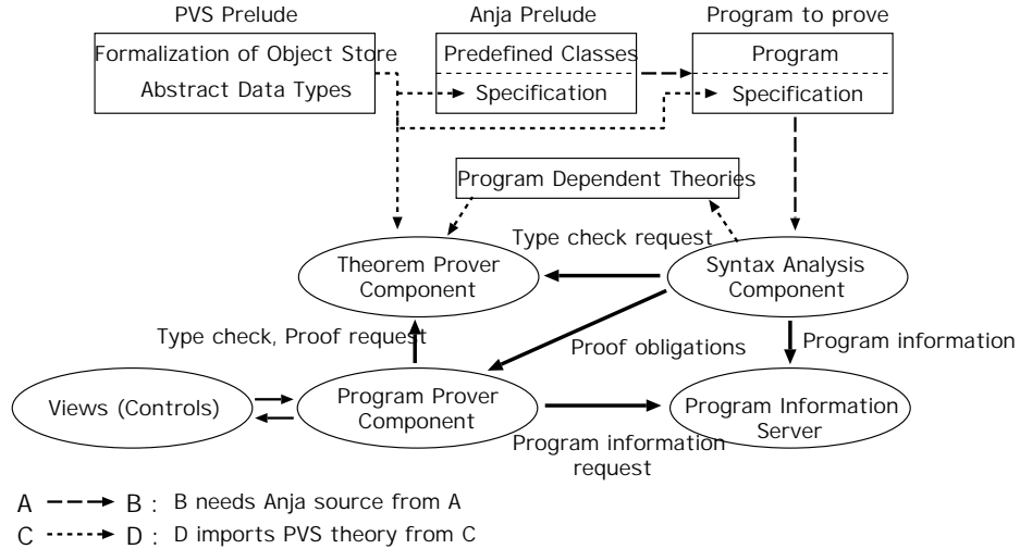
Fig. 2. The JIVE architecture
